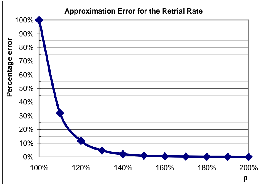
Figure 4: Percentage error of the fluid approximation for the retrieval rate as a function of the number of the system load \rho for C = 40
