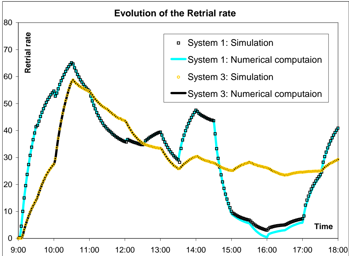
Figure 8: Comparison of simulation results and numerical analysis results for Systems 1 and 3
