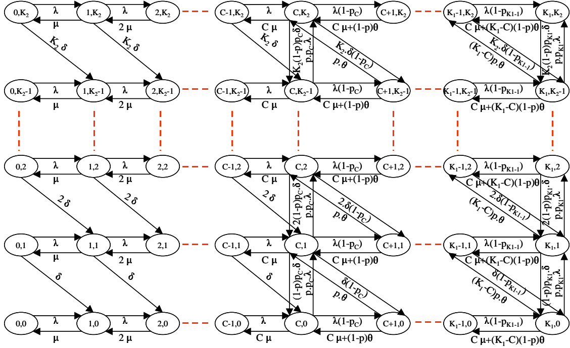
Figure 1: The Transition Diagram of the Markov Chain
