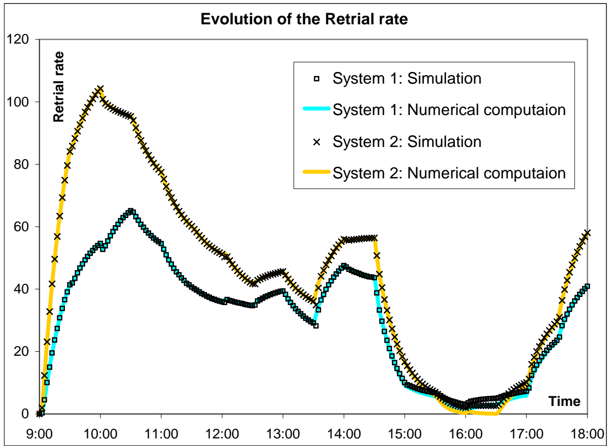
Figure 7: Comparison of simulation results and numerical analysis results for Systems 1 and 2
