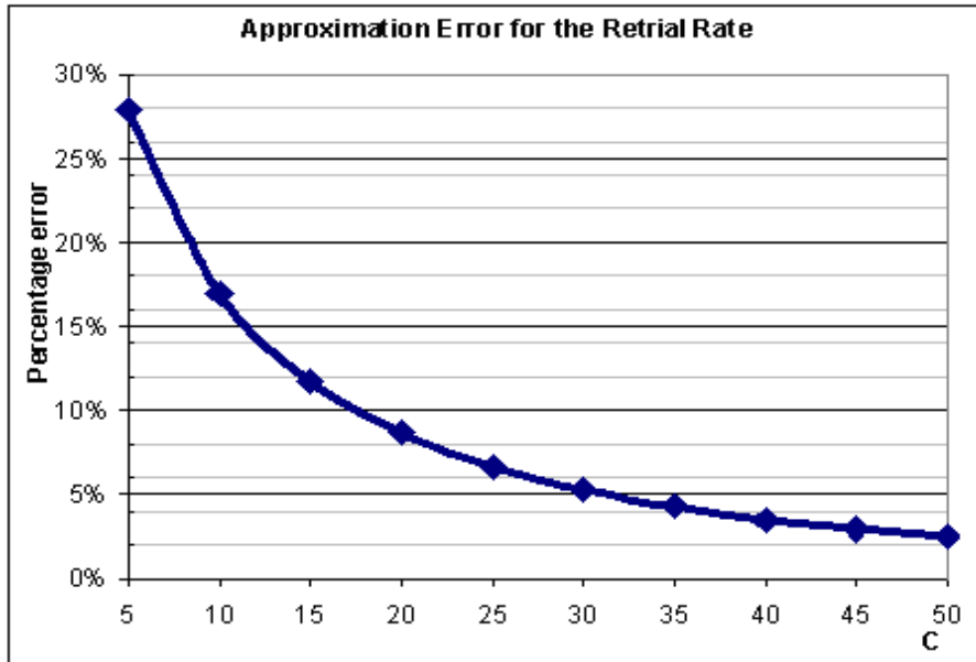
Figure 3: Percentage error of the fluid approximation for the retrieval rate as a function of the number of servers C for \rho = 133\%
