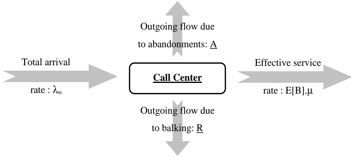
Figure 2: The Incoming and Outgoing Flows
