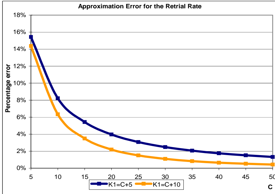
Figure 5: Percentage error of the fluid approximation for the retrial rate as a function of the number of servers C for \rho = 133\% in a system with finite queue capacity
