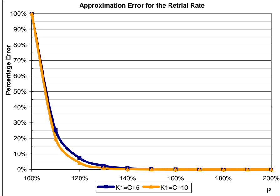
Figure 6: Percentage error of the fluid approximation for the retrieval rate as a function of the number of the system load \rho for C = 40 in a system with finite queue capacity
