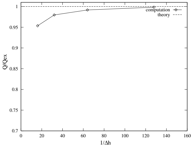
Fig. 2. Resolution test for the validation problem in Fig. 1. Total mass flux scaled by the exact mass flux versus grid resolution.
