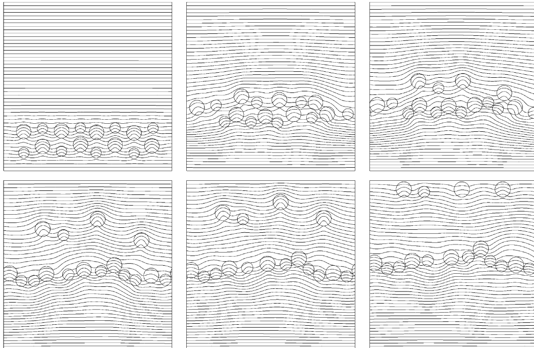
Fig. 11. Isotherms for selected frames from the simulation of 16 two-dimensional unequal size drop interaction. Time progresses from left to right, top to bottom and 50 equally spaced contours are shown. The non-dimensional times ( t^* ) are 4, 64.7, 89, 137.6, 161.9, 202.4. The computational domain is (x/a_v, z/a_v) = (13.33, 13.33) . The non-dimensional numbers based on dimensions of large drops are Re = 5 , Ma = 20 , We = 0.0833 and the material property ratios are 0.5. The ratio of drop radii is \lambda = 5/7 .
